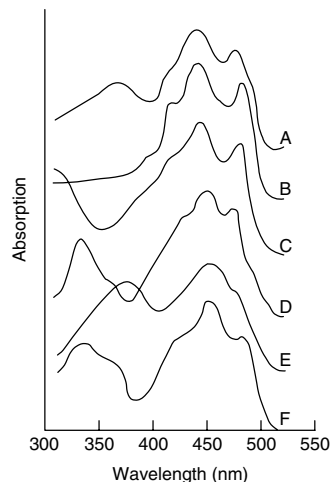
Fig. 12.14 The action spectrum of phototropism in the Avena coleoptile compared with flavins and carotenoids. (A) phototropic action spectrum; (B) \alpha -carotene in hexane; (C) 9-9' cis - \beta -carotene in hexane; (D) hexane extract of 50 Avena coleoptile tips; (E) riboflavin in water; (F) 3-methyl-lumiflavin in benzene. From Thimann & Curry (1961).
